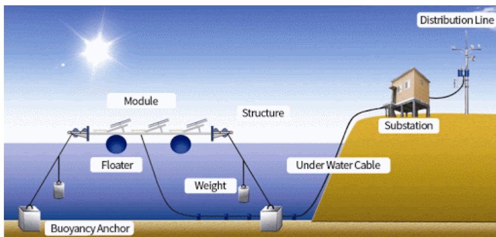
Fig -2: Floating PV plant outline
