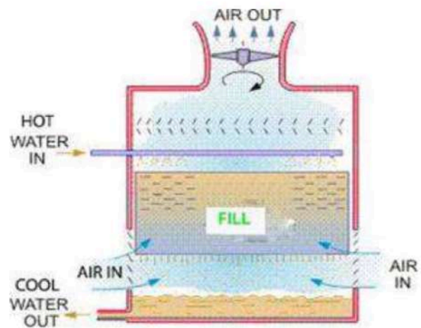
Fig -1: Cooling tower
